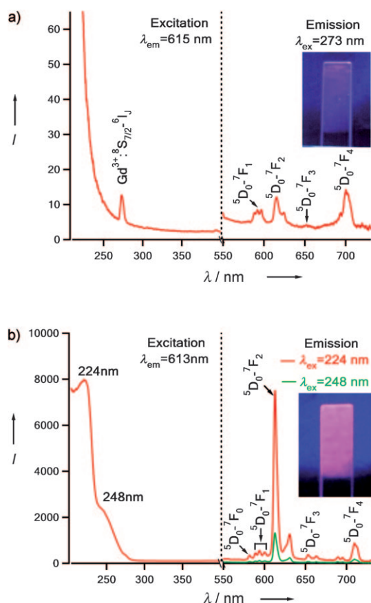
Figure 3. Excitation and emission spectra of a) \text{Gd}(\text{OH})_{2.5}\text{Cl}_{0.5} \cdot 0.9 \text{H}_2\text{O} : 0.05 \text{Eu} film and b) \text{Gd}_2\text{O}_3 : 0.05 \text{Eu} film transformed at 800^\circ\text{C} . The inset shows the red-light emission of the precursor hydroxide film and oxide film under UV irradiation.
